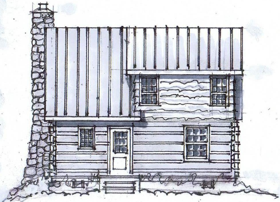
REAR ELEVATION - COKER CREEK
