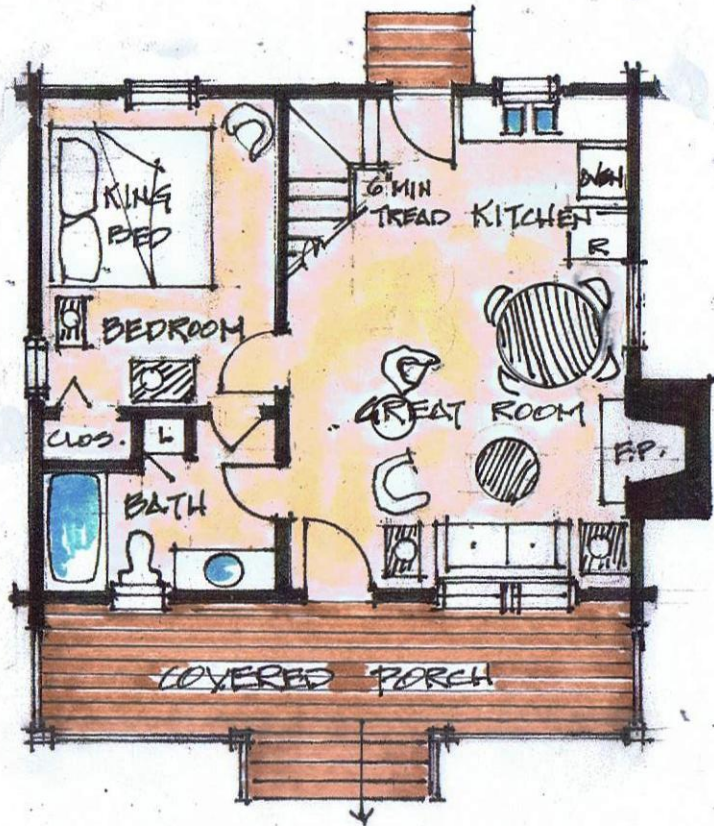
MAIN LEVEL PLAN COKER CREEK
