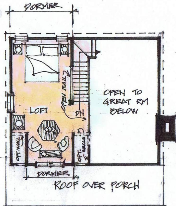
UPPER LEVEL PLAN COKER CREEK
